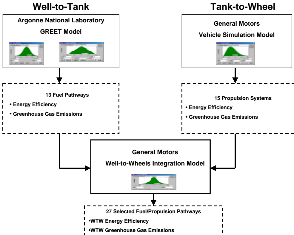
Figure ES-3.1 Well-to-Wheels Integration Process
