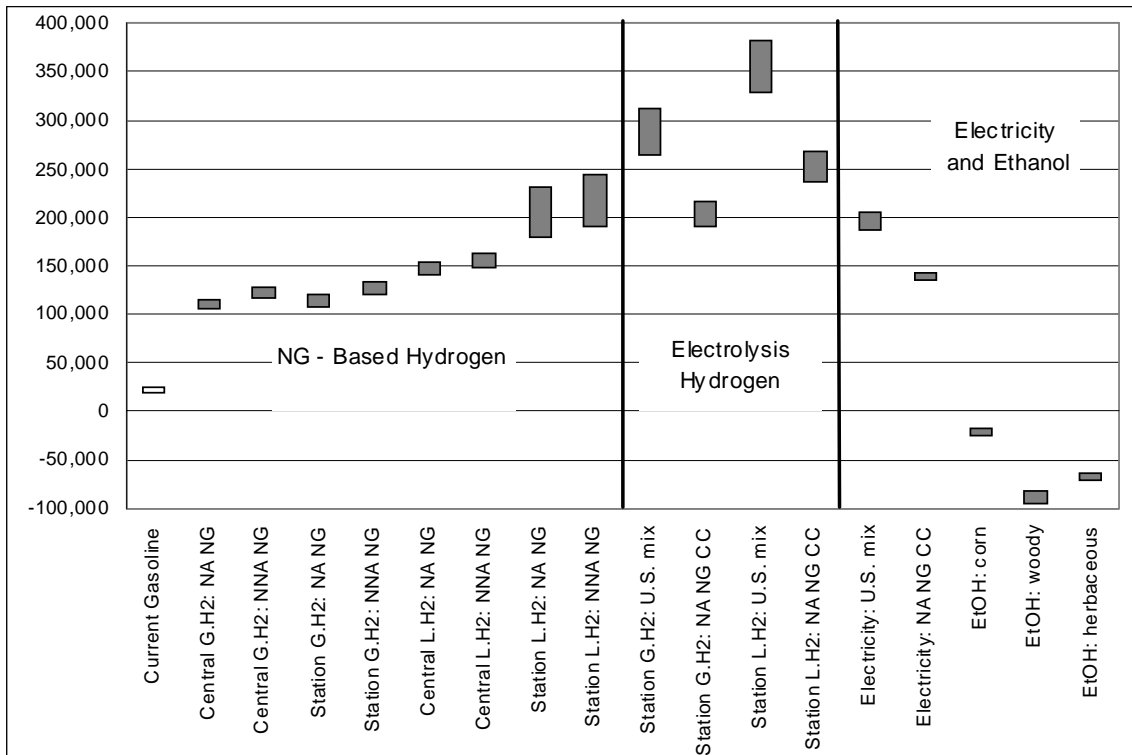
Figure ES-1.4 WTT GHG Emissions: grams per MMBtu of Fuel Delivered to Vehicle Tanks
