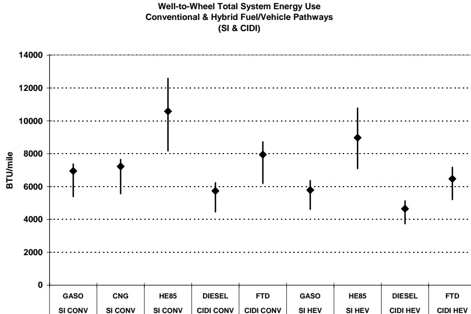
Figure ES-3.2 WTW Total System Energy Use: Conventional and Hybrid Fuel/Vehicle Pathways (SI and CIDI)
