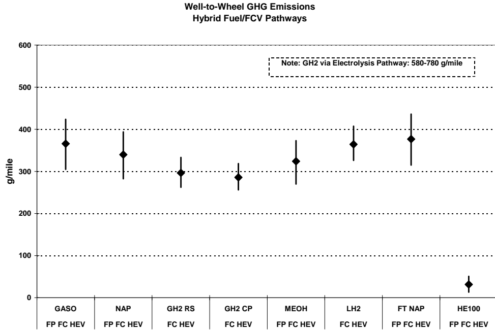
Figure ES-3.5 WTW GHG Emissions: Hybrid Fuel/FCV Pathways
