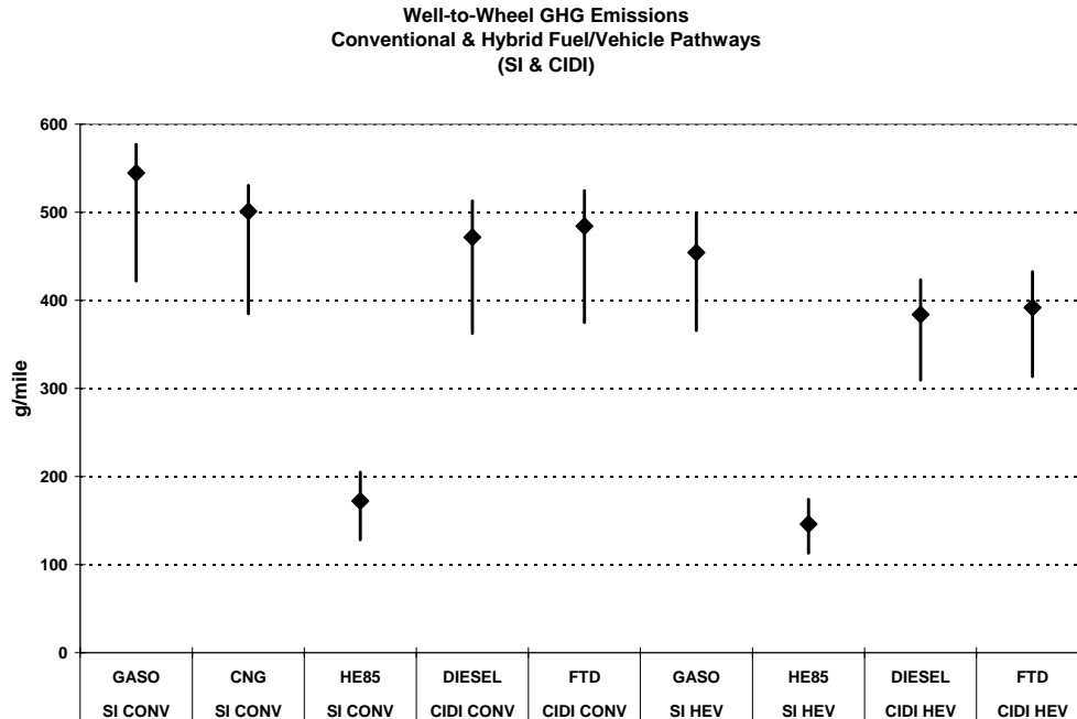
Figure ES-3.3 WTW GHG Emissions: Conventional and Hybrid Fuel/Vehicle Pathways (SI and CIDI)
