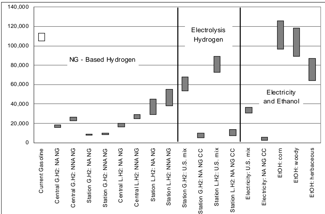
Figure ES-1.3 WTT Petroleum Use: Btu per MMBtu of Fuel Delivered to Vehicle Tanks
