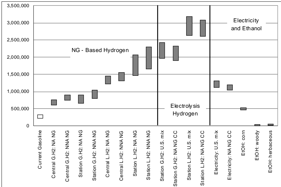
Figure ES-1.2 WTT Fossil Energy Use: Btu per MMBtu of Fuel Delivered to Vehicle Tanks
