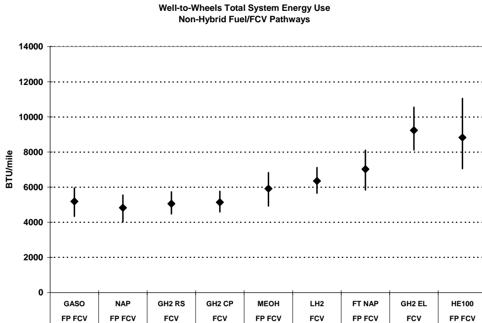
Figure ES-3.6 WTW Total System Energy Use: Non-Hybrid Fuel/FCV Pathways
