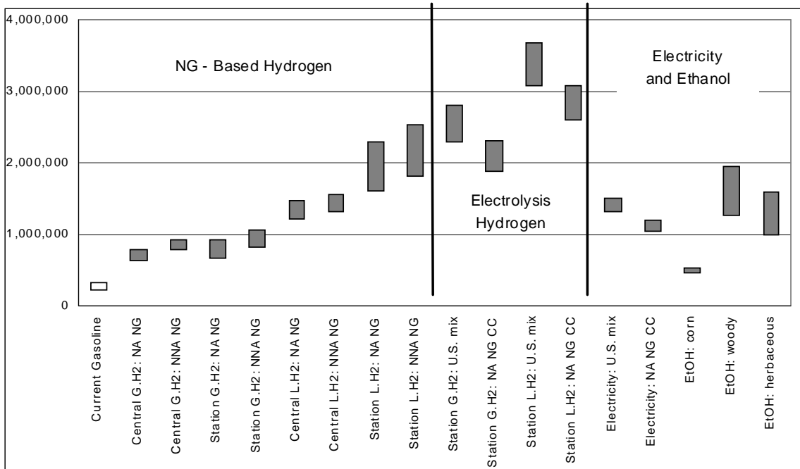
Figure ES-1.1 WTT Total Energy Use: Btu per MMBtu of Fuel Delivered to Vehicle Tanks
